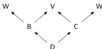
Figure 1 — Name lookup [fig:class.lookup]
